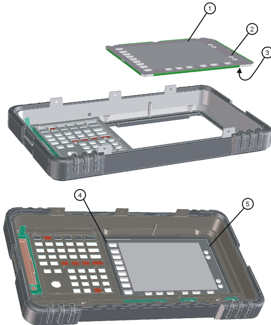
Figure 1 Installing the Lens/Keypad Assembly
